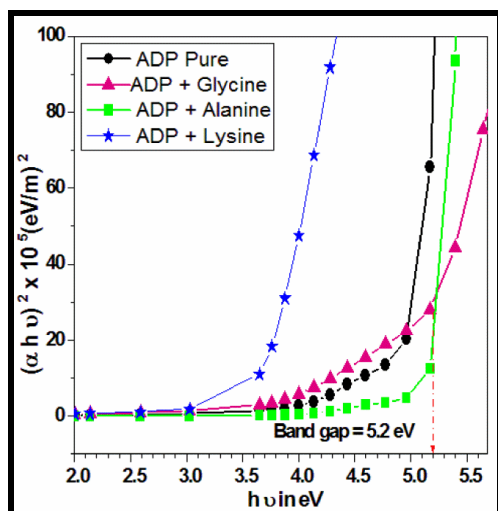
Fig.3 (\alpha hv)^2 vs. h\nu in eV
