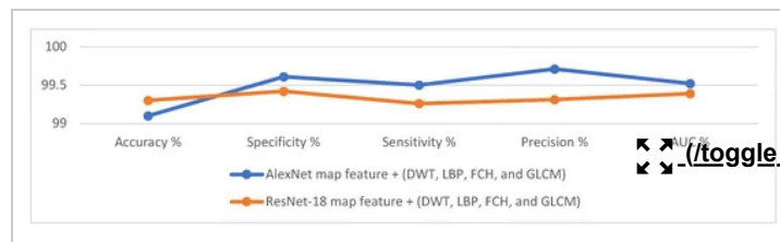
Figure 13. ANN performance based on the hybrid features between CNN models and traditional algorithms.
