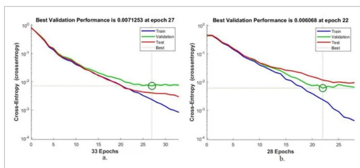
Figure 11. Best validation for evaluating ANN performance based on hybrid features. (a) AlexNet, DWT, LBP, FCH, and GLCM; (b) ResNet-18, DWT, LBP, FCH, and GLCM.
