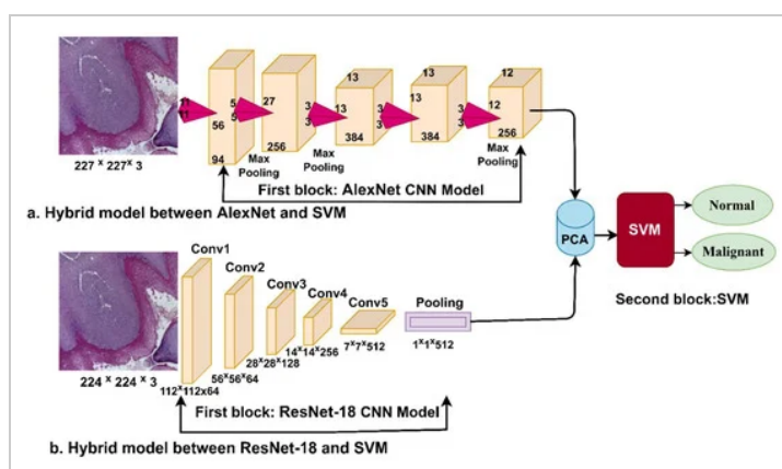
Figure 3. Methodology for histopathological image diagnosis of oral cancer by a hybrid technique between CNN and SVM models.
