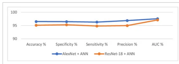
Figure 14. Display of ANN performance based on the features of AlexNet and ResNet-18 models.
