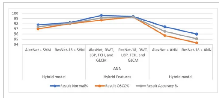
Figure 16. Performance of the proposed methods for OSCC data set diagnostics.
