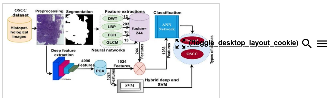
Figure 1. Structure of the histopathological image diagnostics methodology for early diagnosis of OSCC.
